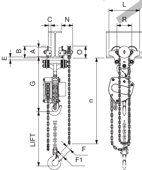
Hoist-Trolley units / Hand driven / Standard type (Art. group 81250-81255)
